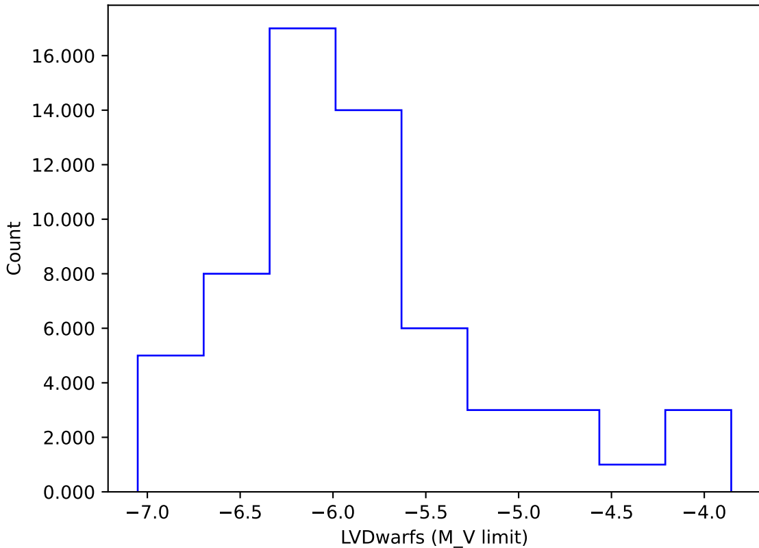
too_elab_r128_d2_ugrizy_v3.4_10yrs gi: LVDwarfs
