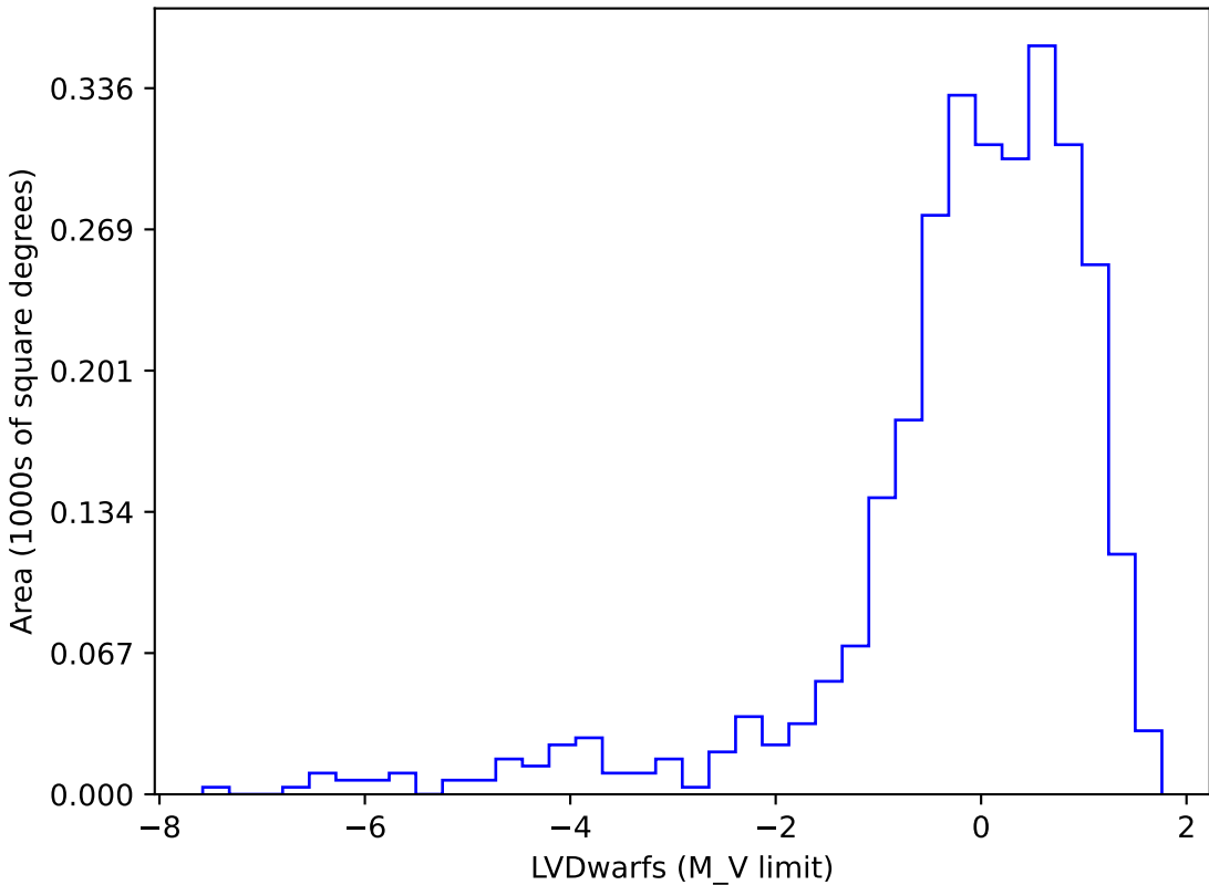
too_elab_r128_d2_ugrizy_v3.4_10yrs gi SCP: LVDwarfs
