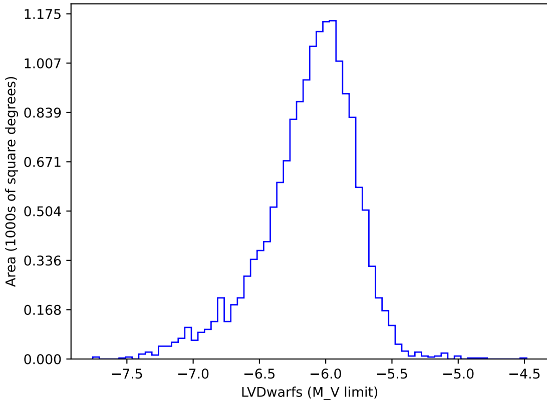
too_elab_r128_d2_ugrizy_v3.4_10yrs gi: LVDwarfs
