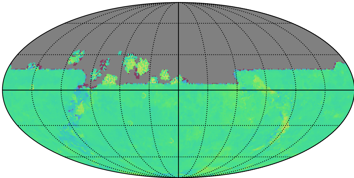
too_elab_r128_d2_ugrizy_v3.4_10yrs u: Kuiper rotTelPos
