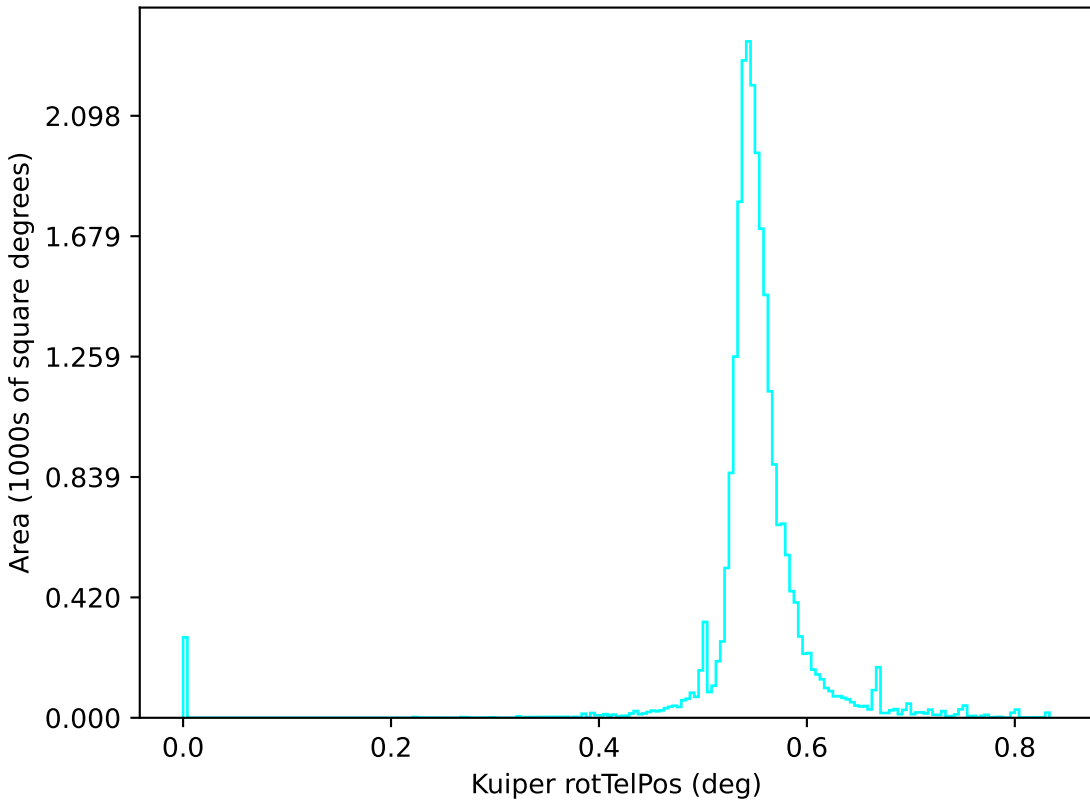
too_elab_r128_d2_ugrizy_v3.4_10yrs u: Kuiper rotTelPos
