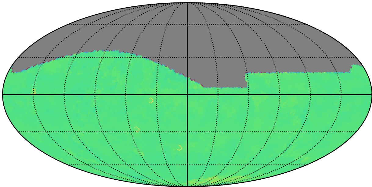
too_elab_r128_d2_ugrizy_v3.4_10yrs r: Kuiper rotTelPos
