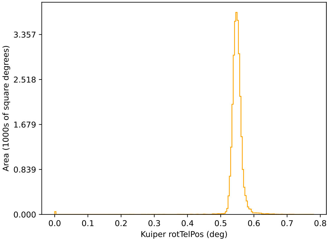
too_elab_r128_d2_ugrizy_v3.4_10yrs r: Kuiper rotTelPos
