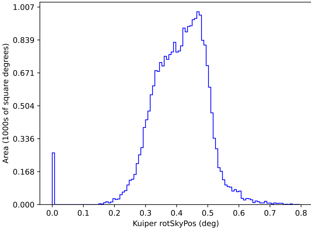
too_elab_r128_d2_ugrizy_v3.4_10yrs y: Kuiper rotSkyPos
