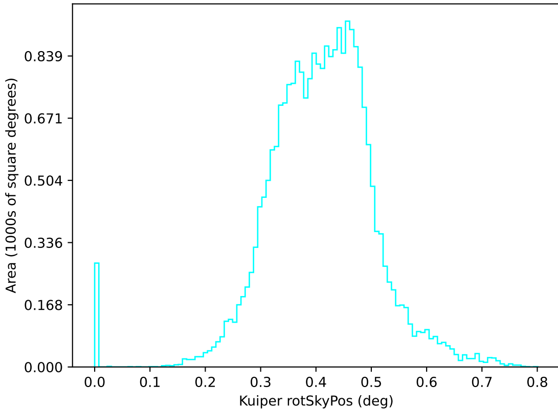
too_elab_r128_d2_ugrizy_v3.4_10yrs u: Kuiper rotSkyPos
