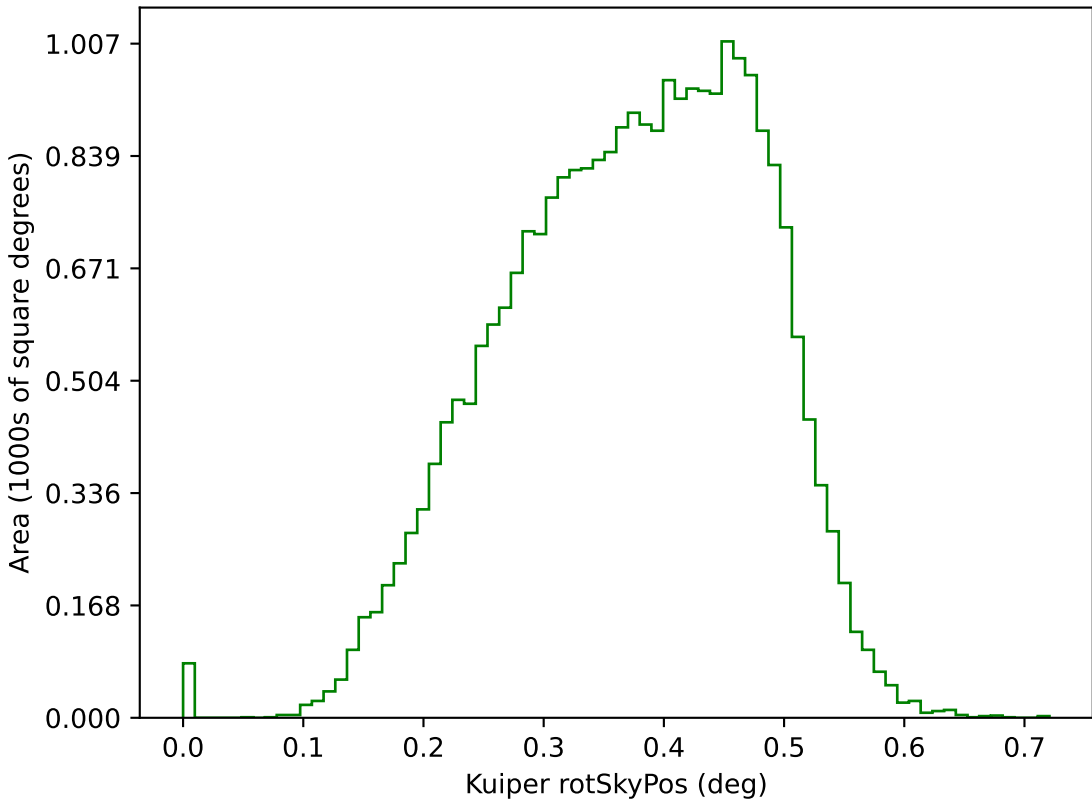
too_elab_r128_d2_ugrizy_v3.4_10yrs g: Kuiper rotSkyPos
