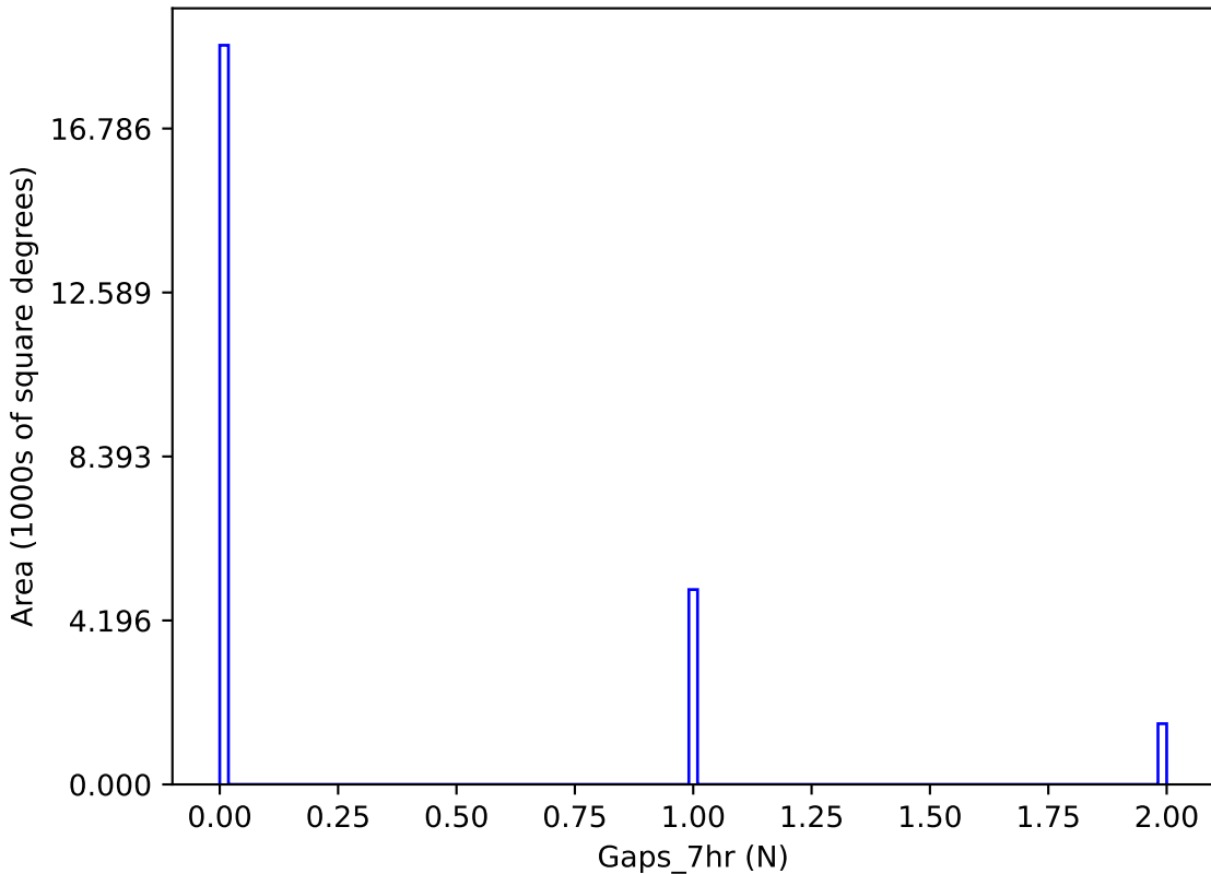
too_elab_r128_d2_ugrizy_v3.4_10yrs y band: Gaps_7hr
