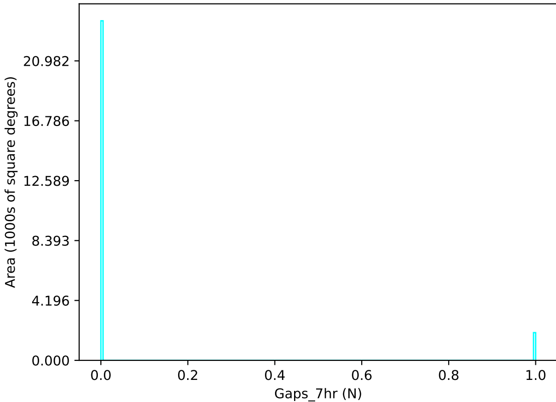
too_elab_r128_d2_ugrizy_v3.4_10yrs u band: Gaps_7hr
