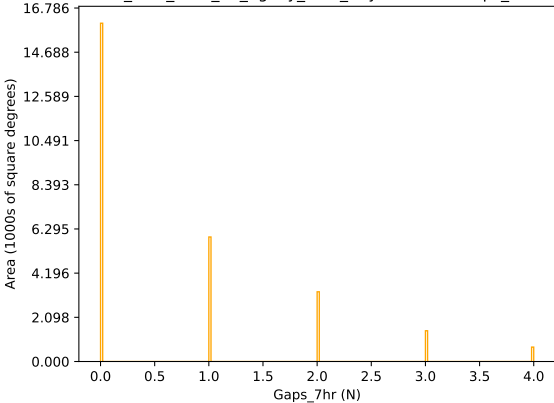
too_elab_r128_d2_ugrizy_v3.4_10yrs r band: Gaps_7hr
