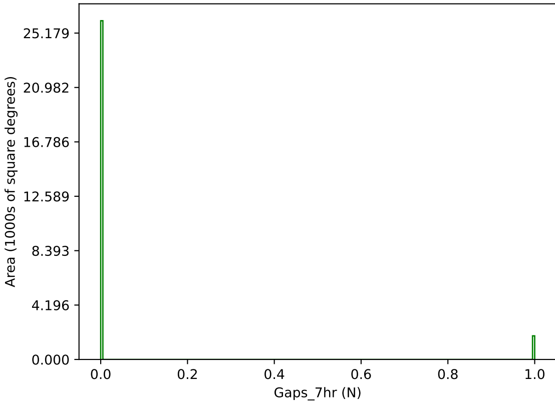
too_elab_r128_d2_ugrizy_v3.4_10yrs g band: Gaps_7hr
