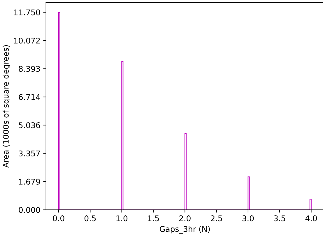
too_elab_r128_d2_ugrizy_v3.4_10yrs z band: Gaps_3hr
