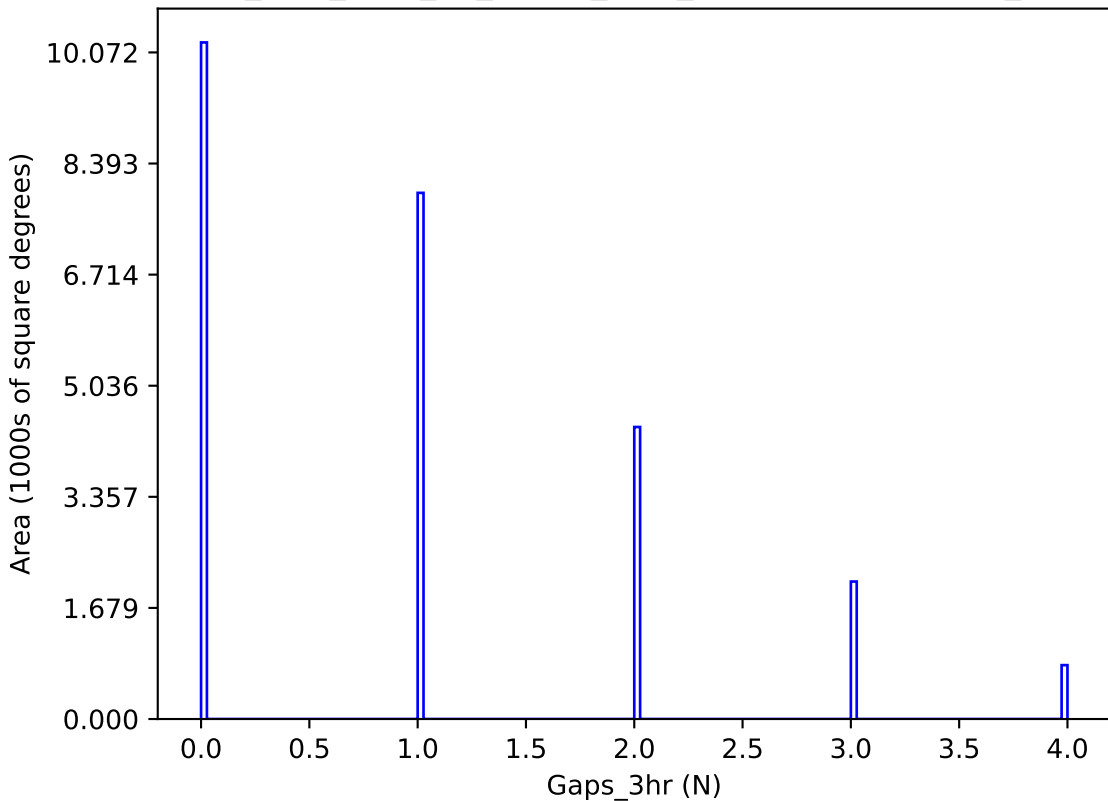
too_elab_r128_d2_ugrizy_v3.4_10yrs y band: Gaps_3hr
