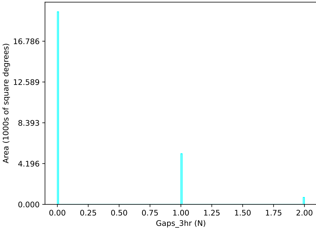
too_elab_r128_d2_ugrizy_v3.4_10yrs u band: Gaps_3hr
