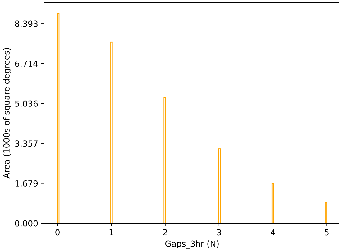
too_elab_r128_d2_ugrizy_v3.4_10yrs r band: Gaps_3hr
