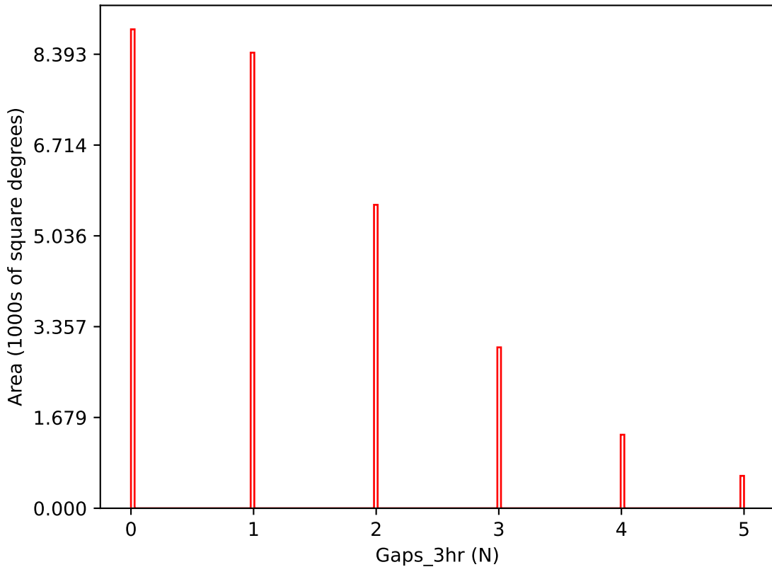
too_elab_r128_d2_ugrizy_v3.4_10yrs i band: Gaps_3hr
