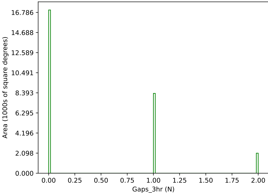
too_elab_r128_d2_ugrizy_v3.4_10yrs g band: Gaps_3hr
