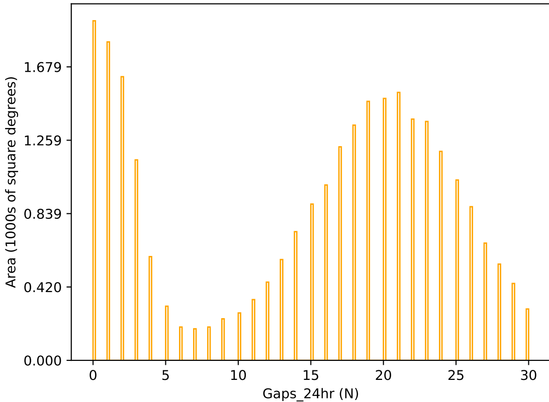
too_elab_r128_d2_ugrizy_v3.4_10yrs r band: Gaps_24hr
