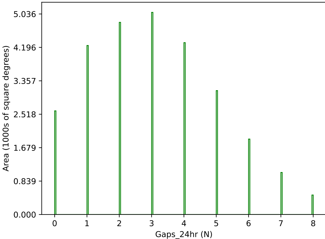
too_elab_r128_d2_ugrizy_v3.4_10yrs g band: Gaps_24hr
