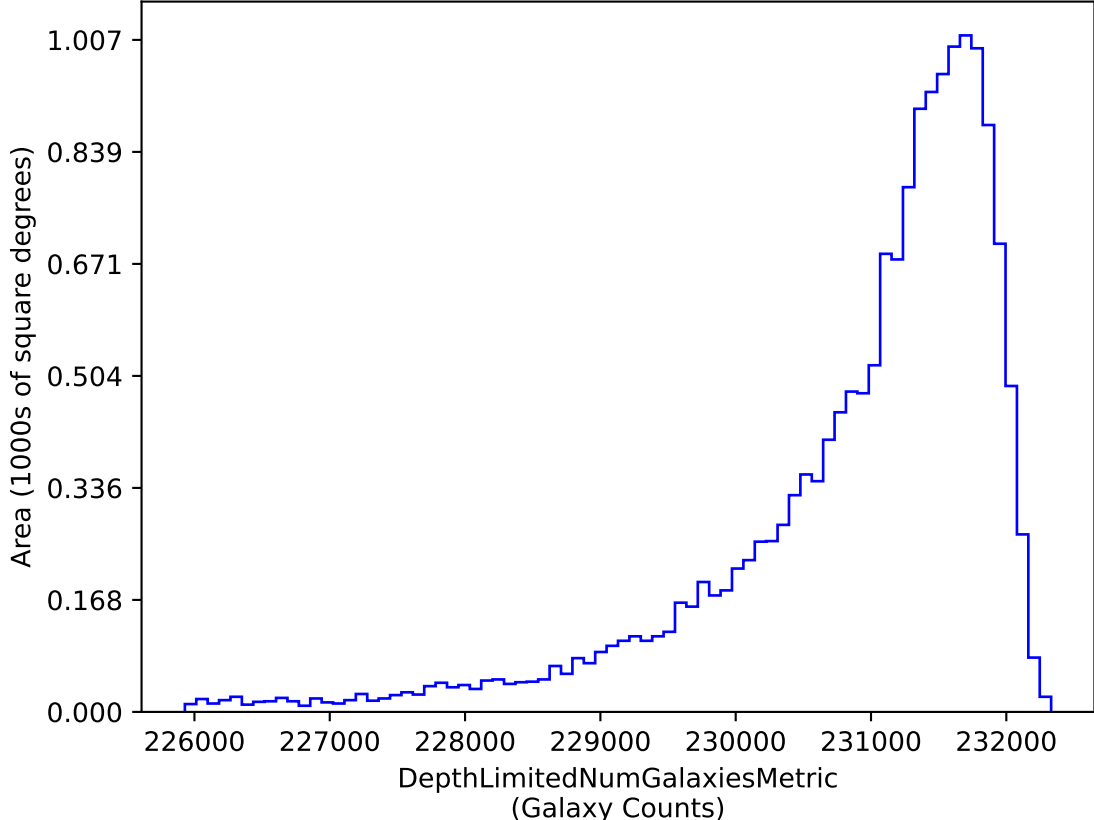
too_elab_r128_d2_ugrizy_v3.4_10yrs i band galaxies non-DD: DepthLimitedNumGalaxiesMetric
