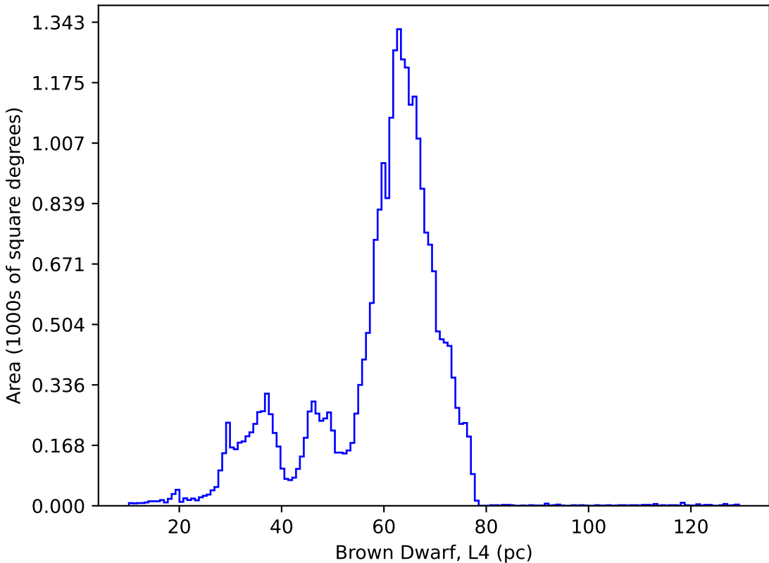
too_elab_r128_d2_ugrizy_v3.4_10yrs : Brown Dwarf, L4
