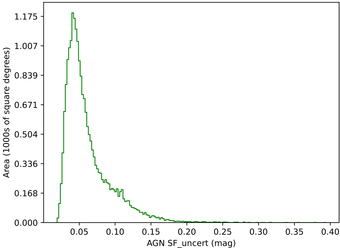
too_elab_r128_d2_ugrizy_v3.4_10yrs g band: AGN SF_uncert
