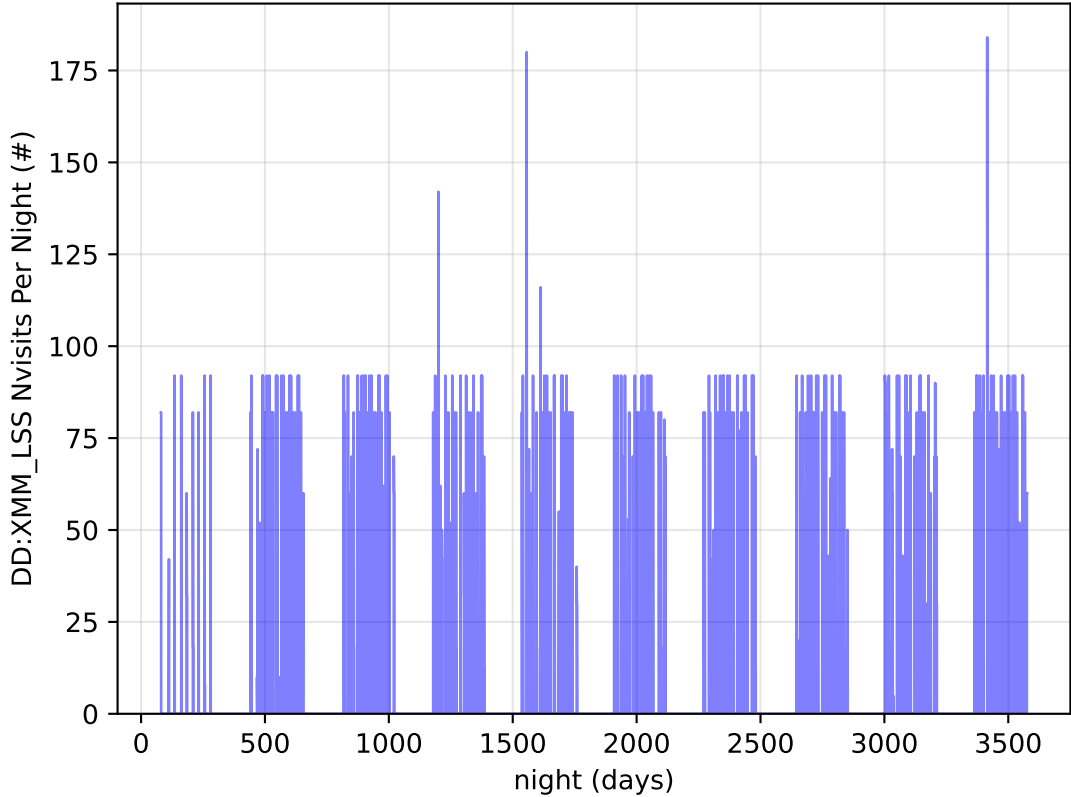
too_elab_r128_d2_ugrizy_v3.4_10yrs all bands: DD:XMM_LSS Nvisits Per Night
