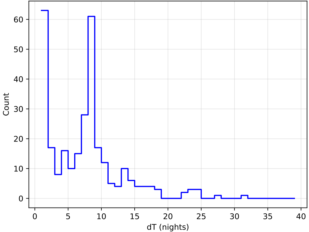
too_elab_r128_d2_ugrizy_v3.4_10yrs all bands: DD:XMM_LSS Delta Nights Histogram
