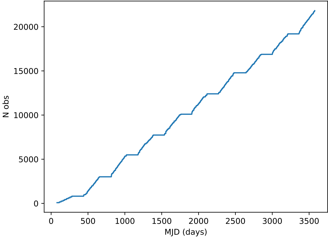
too_elab_r128_d2_ugrizy_v3.4_10yrs all bands: DD:XMM_LSS Cumulative NVisits
