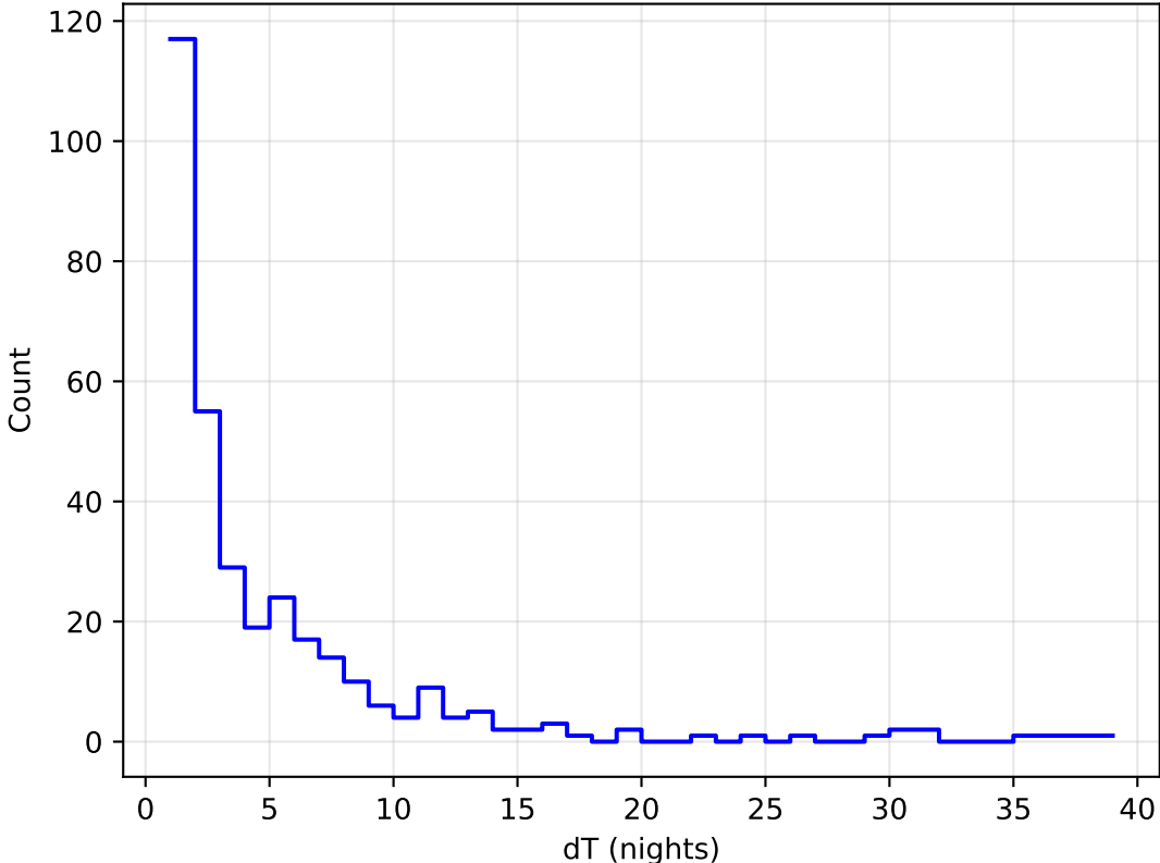
too_elab_r128_d2_ugrizy_v3.4_10yrs all bands: DD:WFD Delta Nights Histogram
