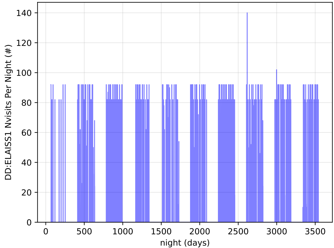
too_elab_r128_d2_ugrizy_v3.4_10yrs all bands: DD:ELAISS1 Nvisits Per Night
