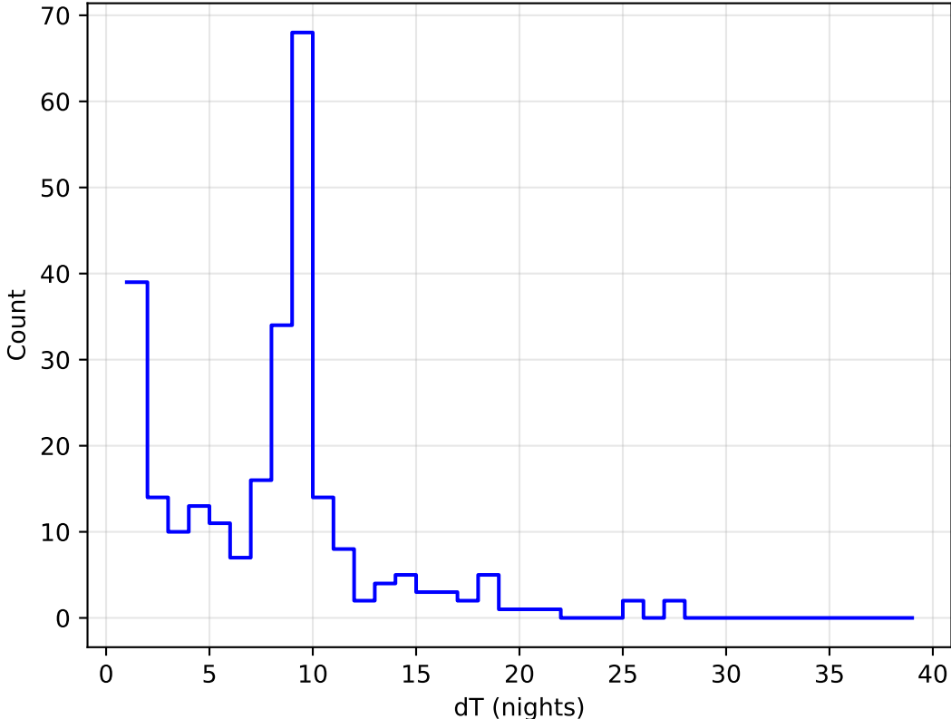
too_elab_r128_d2_ugrizy_v3.4_10yrs all bands: DD:ELAISS1 Delta Nights Histogram
