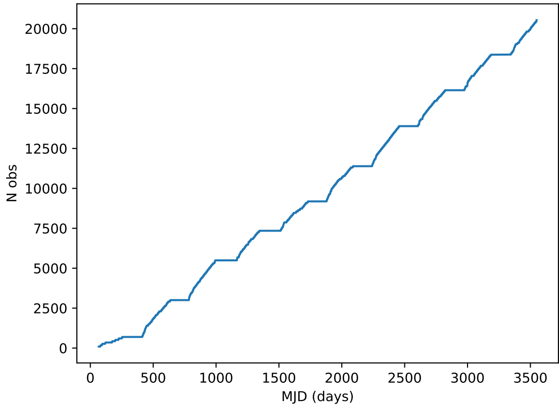
too_elab_r128_d2_ugrizy_v3.4_10yrs all bands: DD:ELAISS1 Cumulative NVisits
