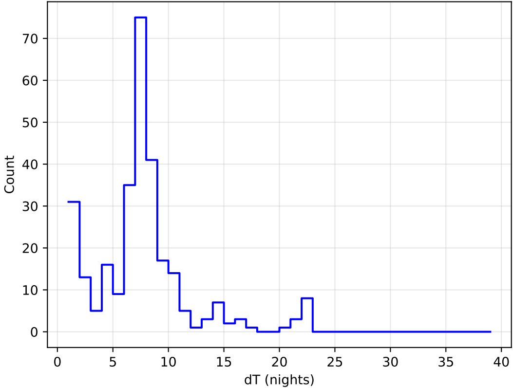
too_elab_r128_d2_ugrizy_v3.4_10yrs all bands: DD:EDFS Delta Nights Histogram
