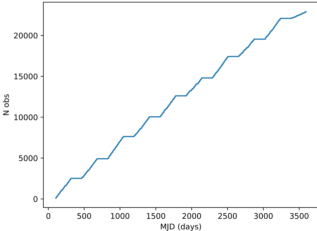
too_elab_r128_d2_ugrizy_v3.4_10yrs all bands: DD:EDFS Cumulative NVisits
