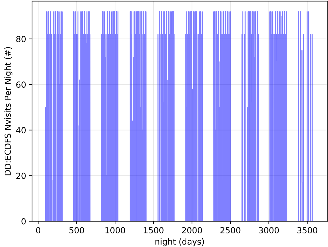
too_elab_r128_d2_ugrizy_v3.4_10yrs all bands: DD:ECDFS Nvisits Per Night
