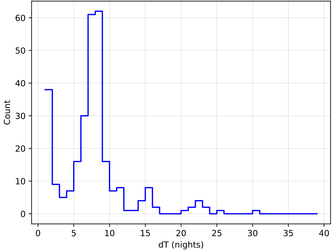
too_elab_r128_d2_ugrizy_v3.4_10yrs all bands: DD:ECDFS Delta Nights Histogram
