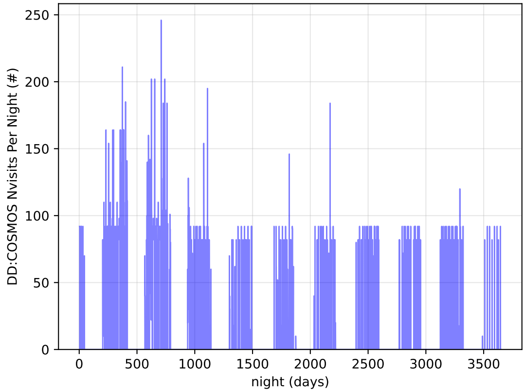
too_elab_r128_d2_ugrizy_v3.4_10yrs all bands: DD: COSMOS Nvisits Per Night
