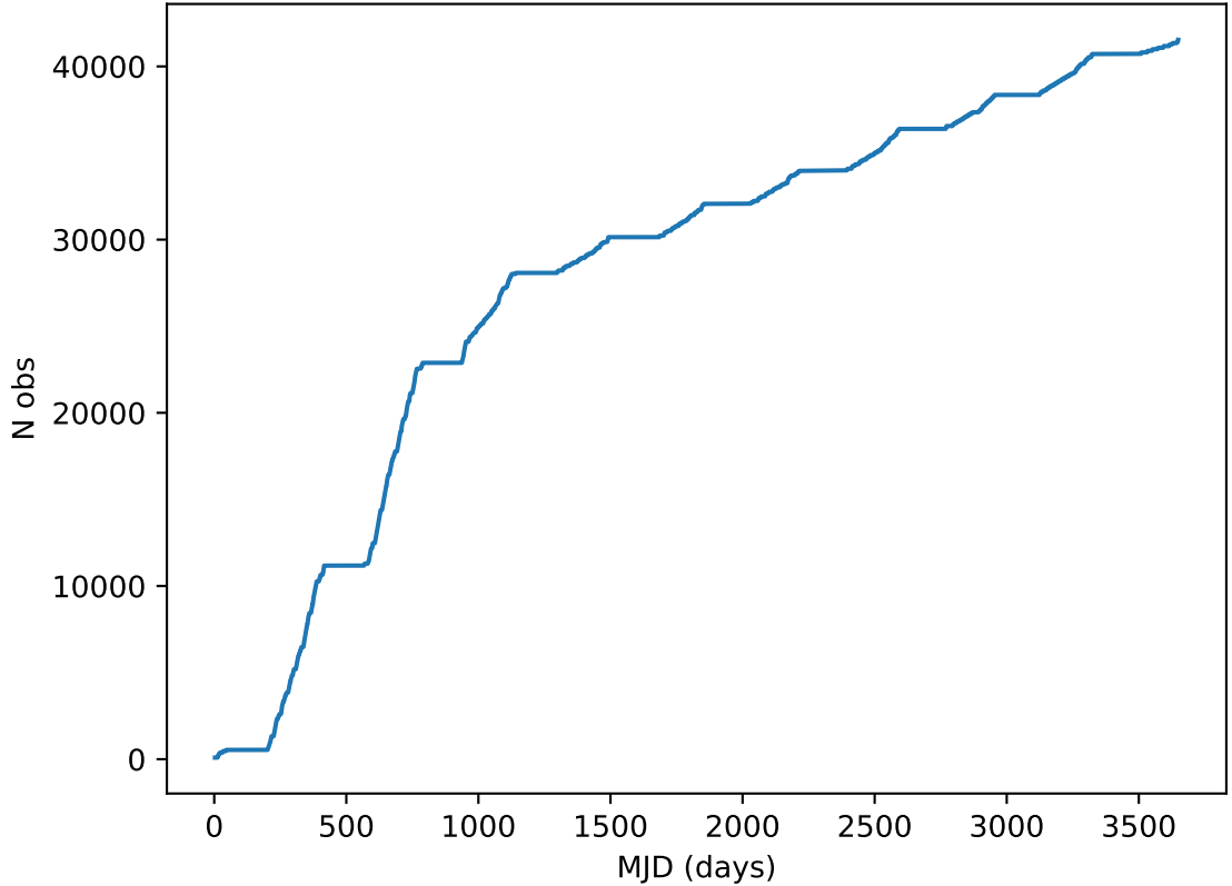
too_elab_r128_d2_ugrizy_v3.4_10yrs all bands: DD:COSMOS Cumulative NVisits
