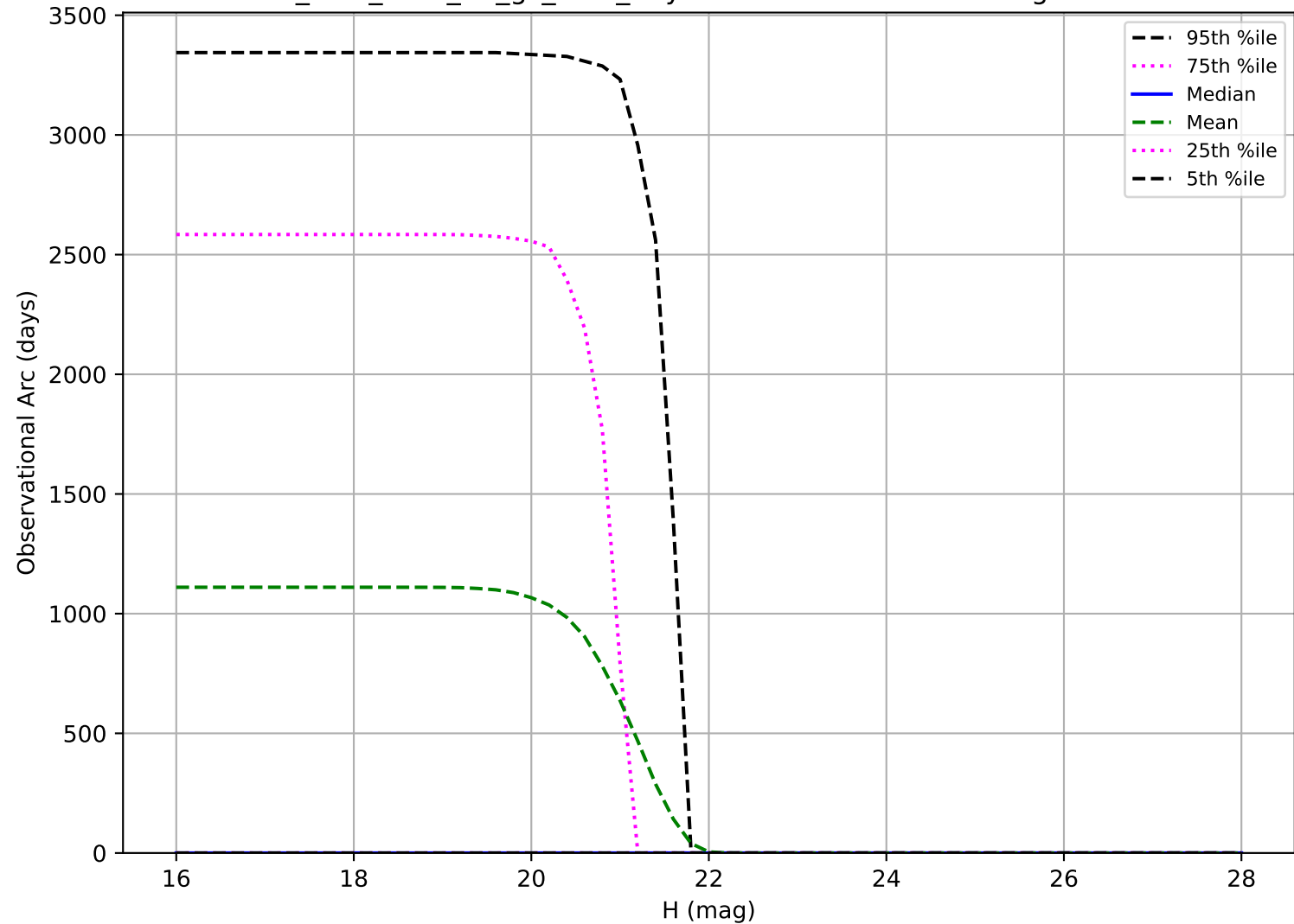
too_elab_r128_d2_gz_v3.4_10yrs: Observational Arc Length Vatira
