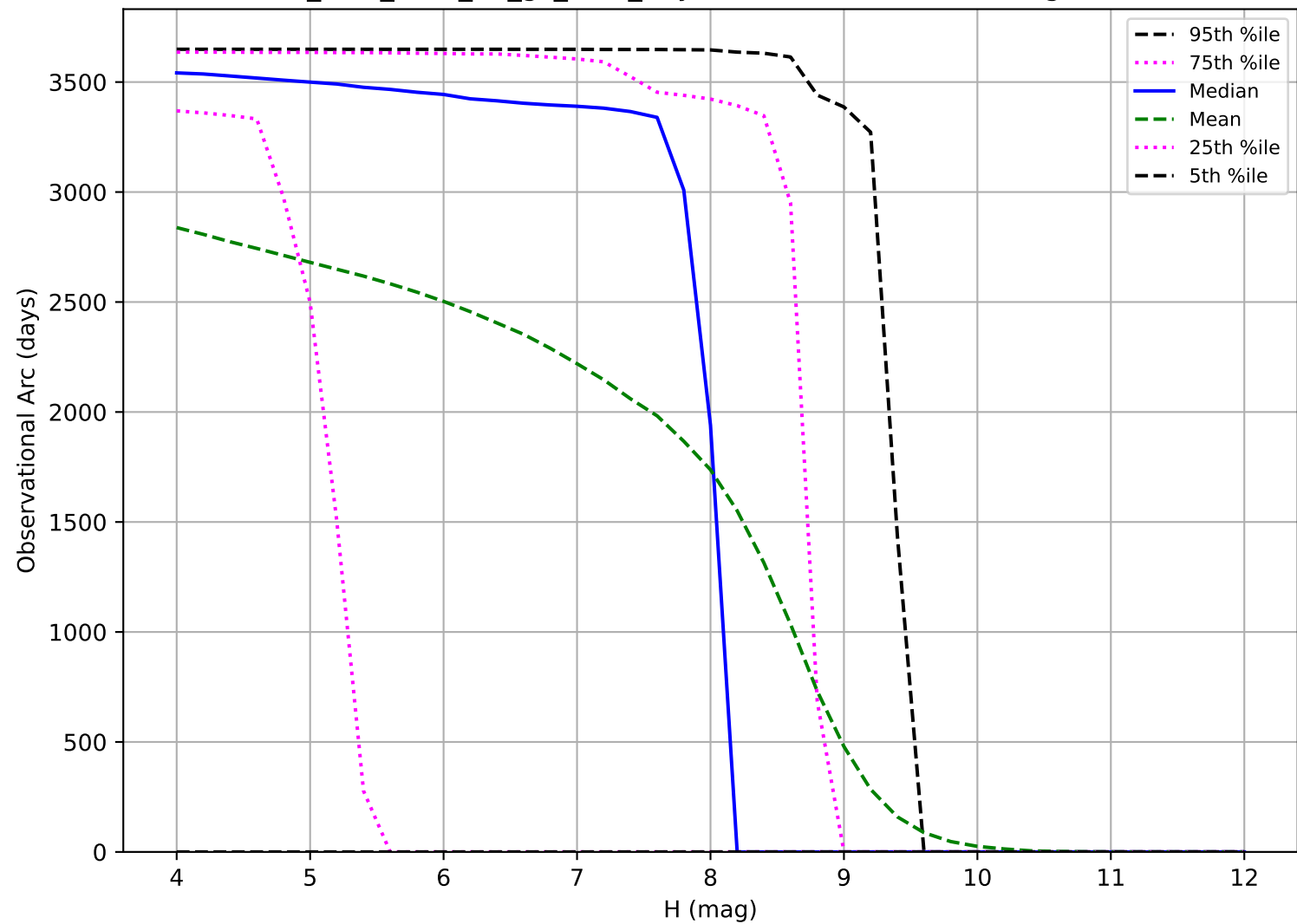
too_elab_r128_d2_gz_v3.4_10yrs: Observational Arc Length TNO
