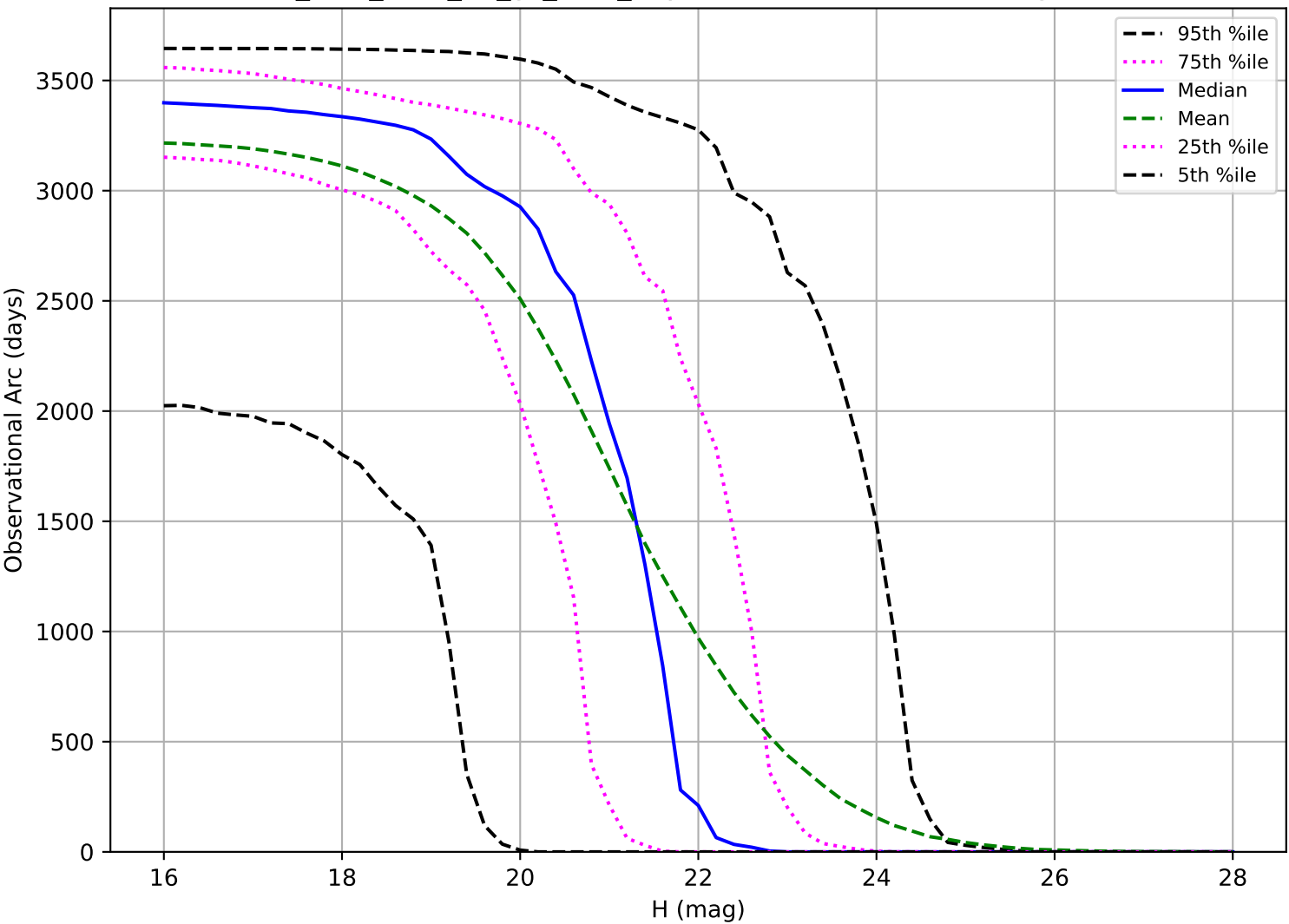
too_elab_r128_d2_gz_v3.4_10yrs: Observational Arc Length PHA
