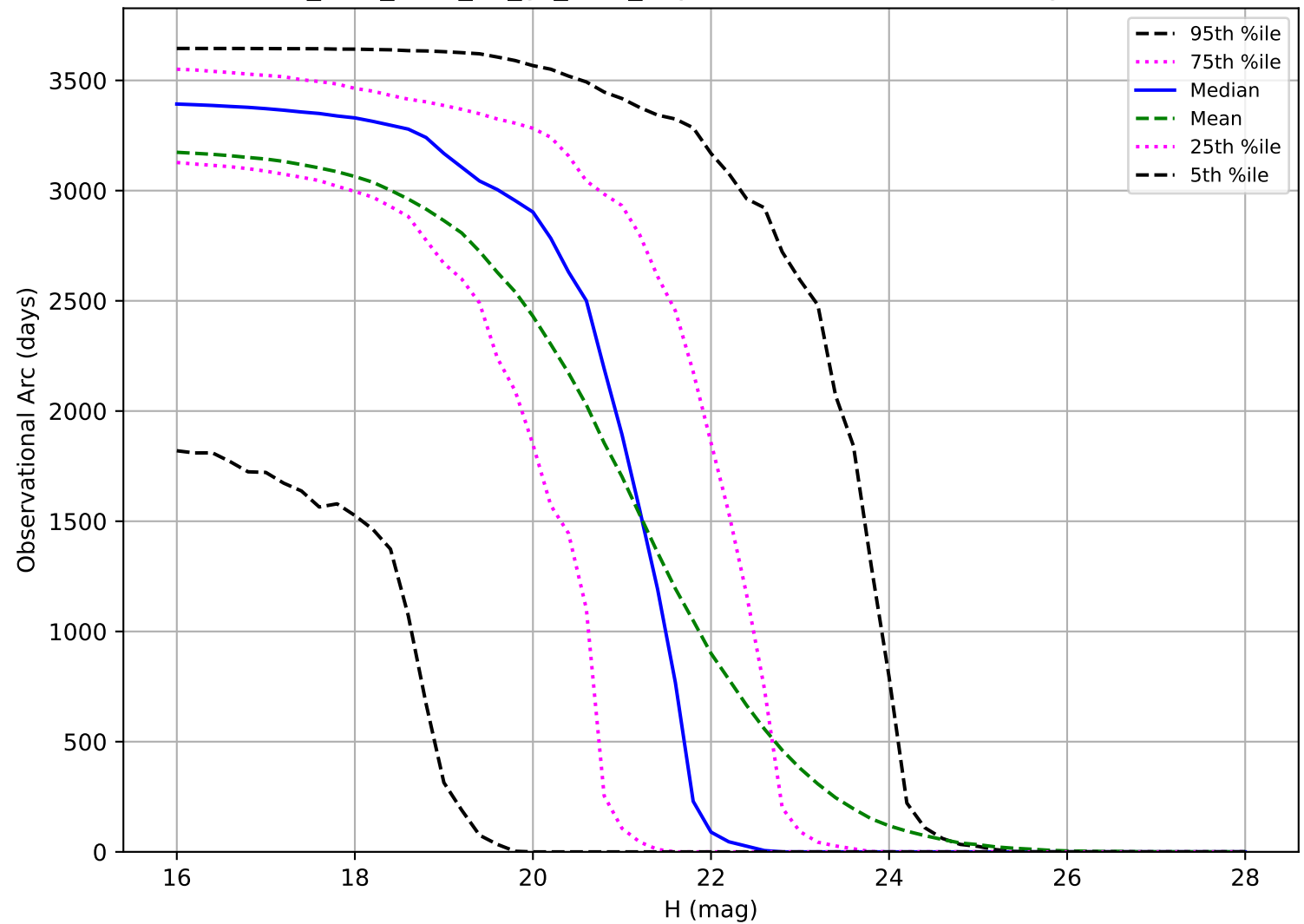
too_elab_r128_d2_gz_v3.4_10yrs: Observational Arc Length NEO
