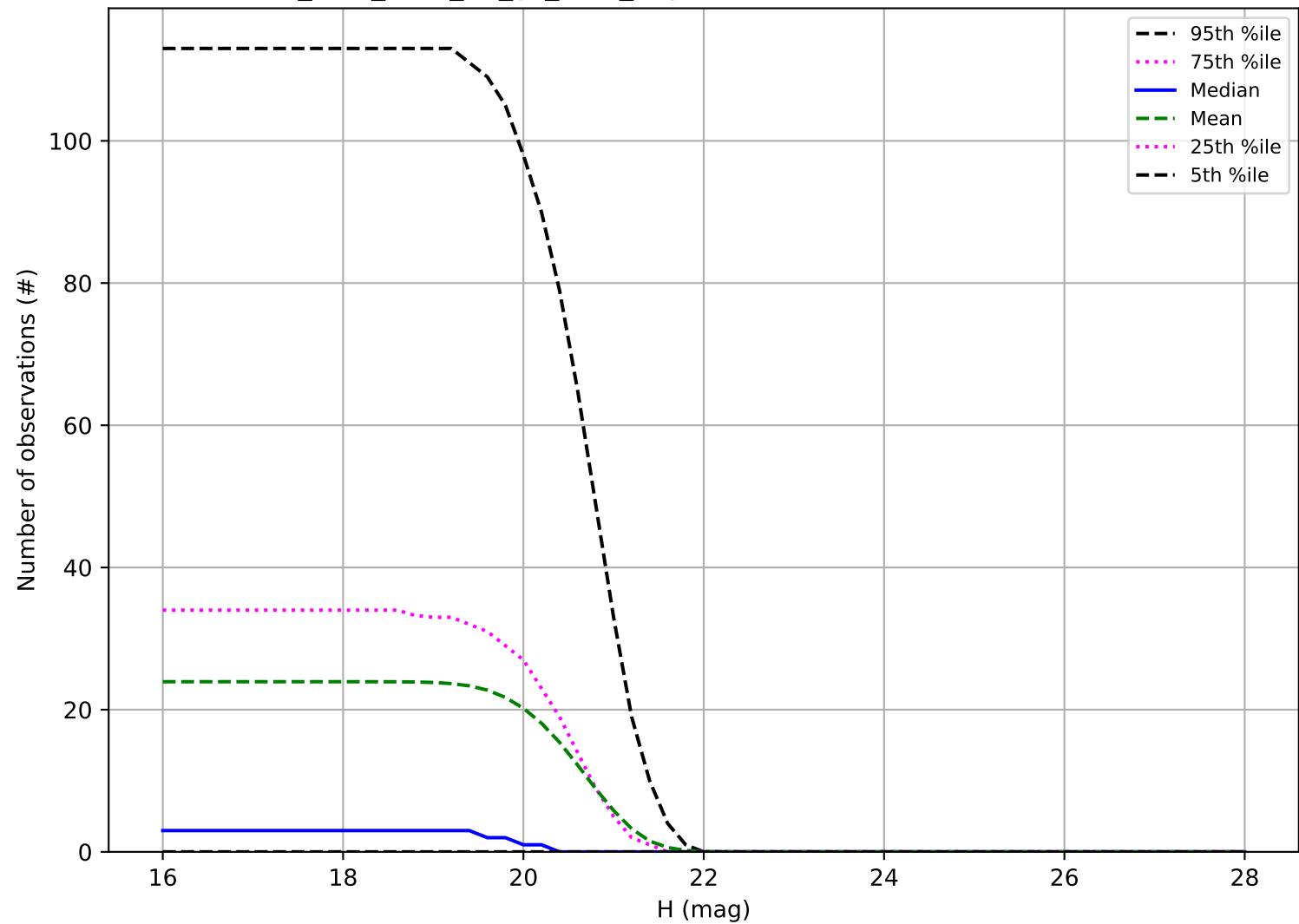
too_elab_r128_d2_gz_v3.4_10yrs: Number of observations Vatira
