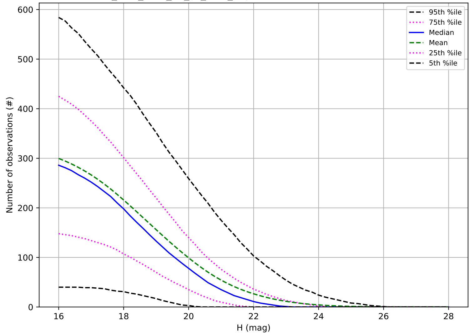
too_elab_r128_d2_gz_v3.4_10yrs: Number of observations PHA
