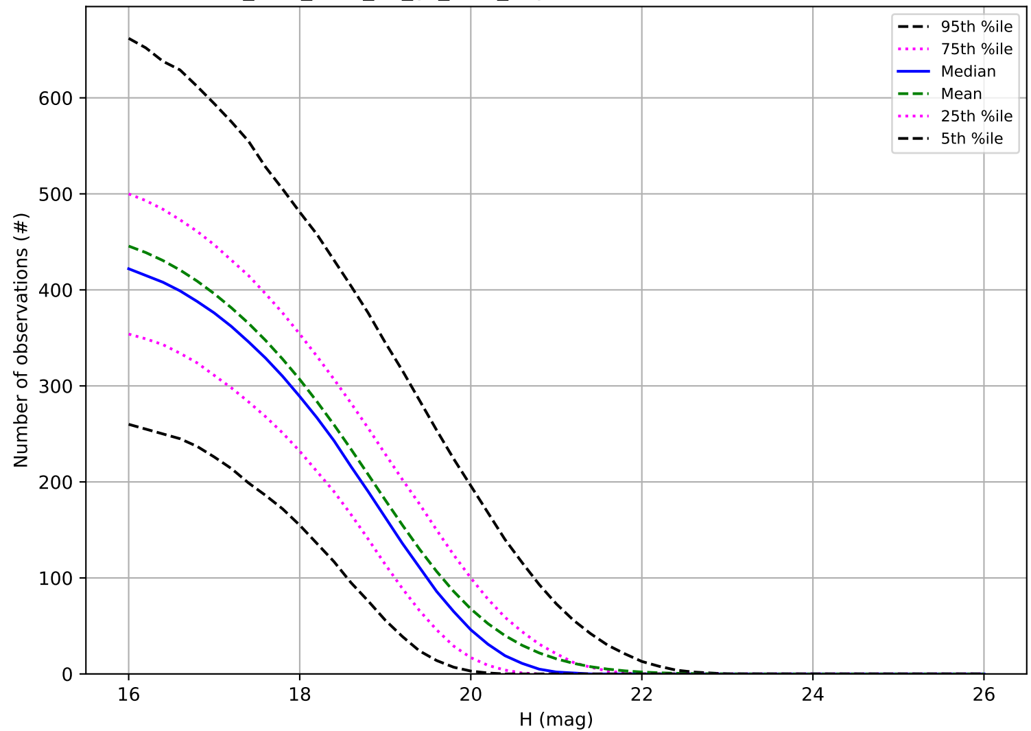
too_elab_r128_d2_gz_v3.4_10yrs: Number of observations MBA
