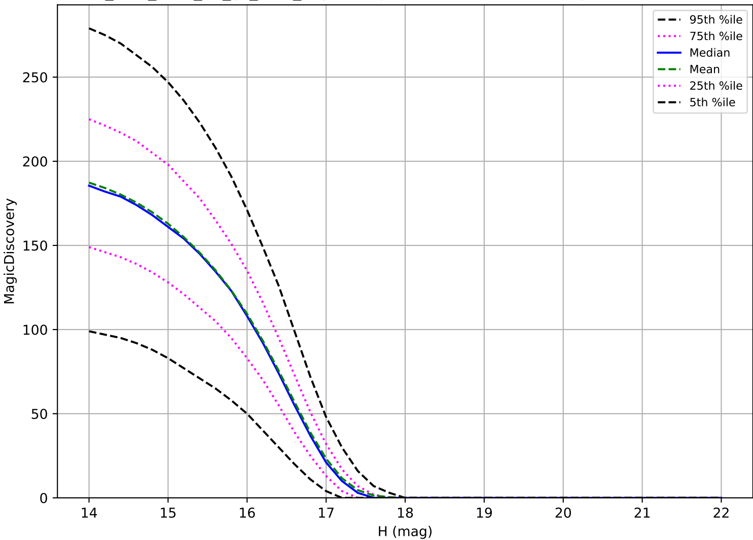
too_elab_r128_d2_gz_v3.4_10yrs: Trojan 6 detections in 60 nights detection loss
