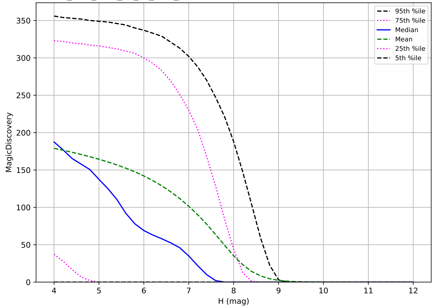
too_elab_r128_d2_gz_v3.4_10yrs: TNO 6 detections in 60 nights detection loss
