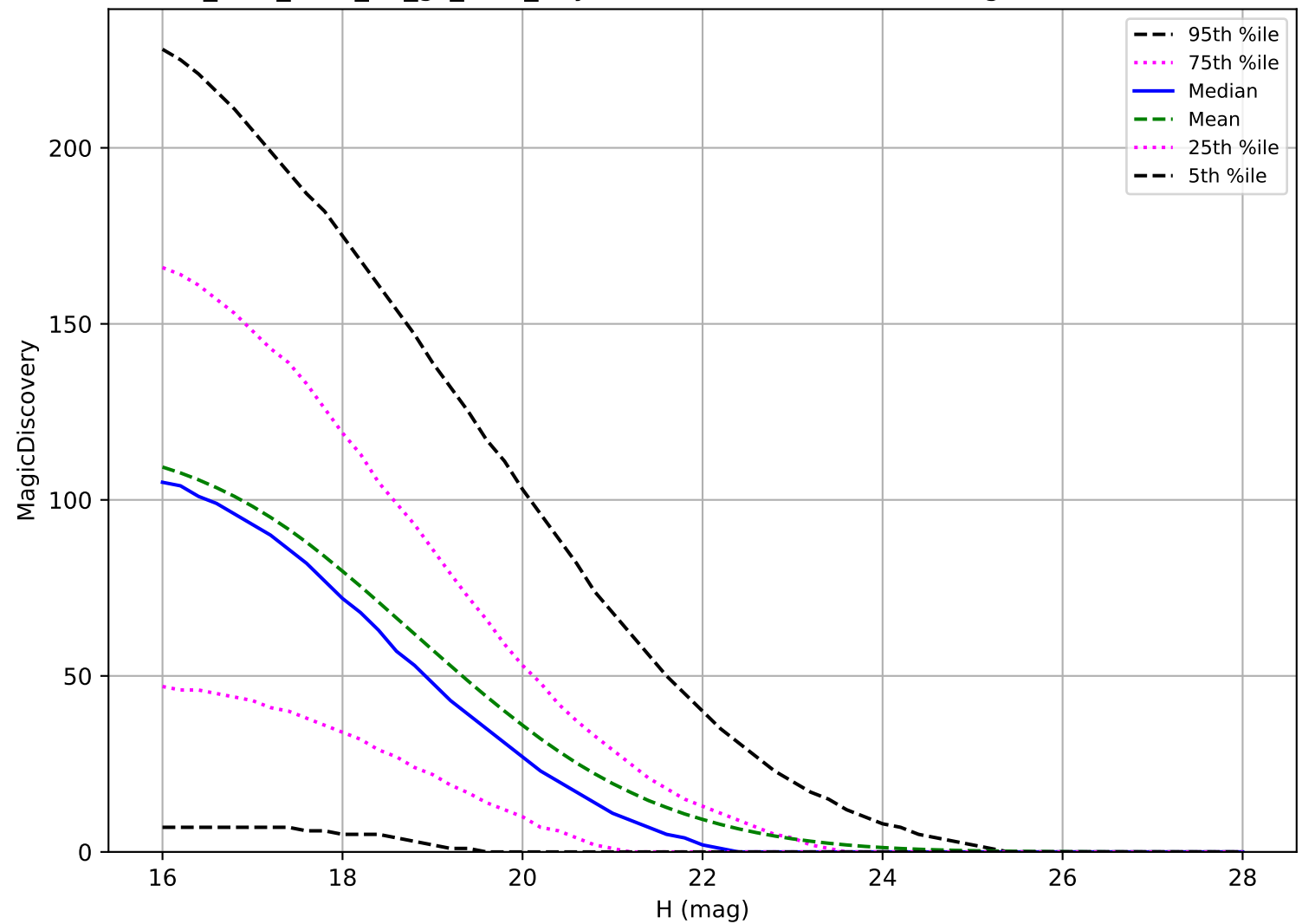
too_elab_r128_d2_gz_v3.4_10yrs: PHA 6 detections in 60 nights detection loss
