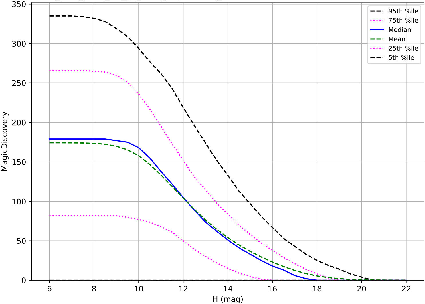
too_elab_r128_d2_gz_v3.4_10yrs: OCC_r5 6 detections in 60 nights detection loss
