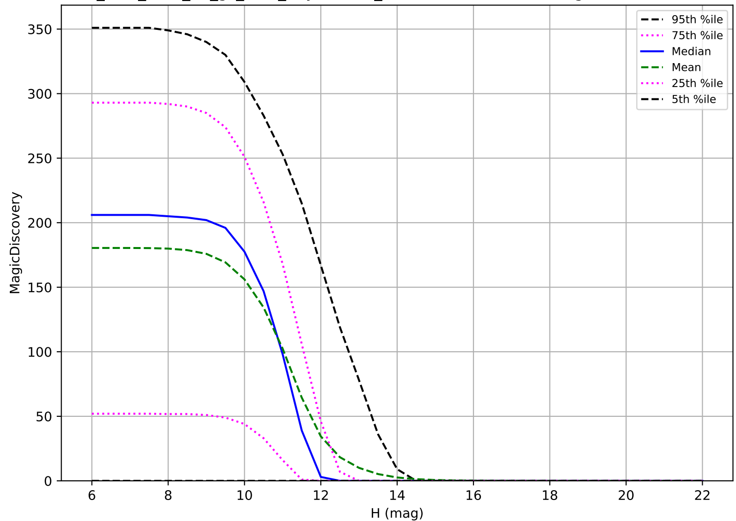
too_elab_r128_d2_gz_v3.4_10yrs: OCC_r20 6 detections in 60 nights detection loss
